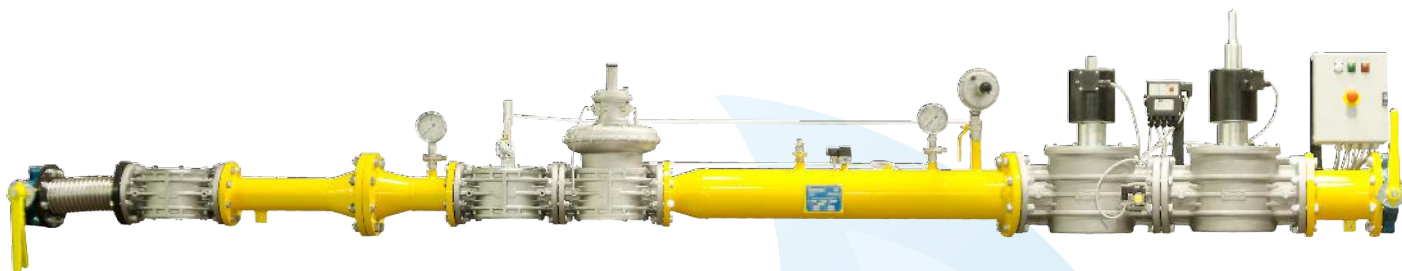
RAMPE GAS CON QUADRO ELETTRICO GAS TRAIN WITH CONTROL PANEL
