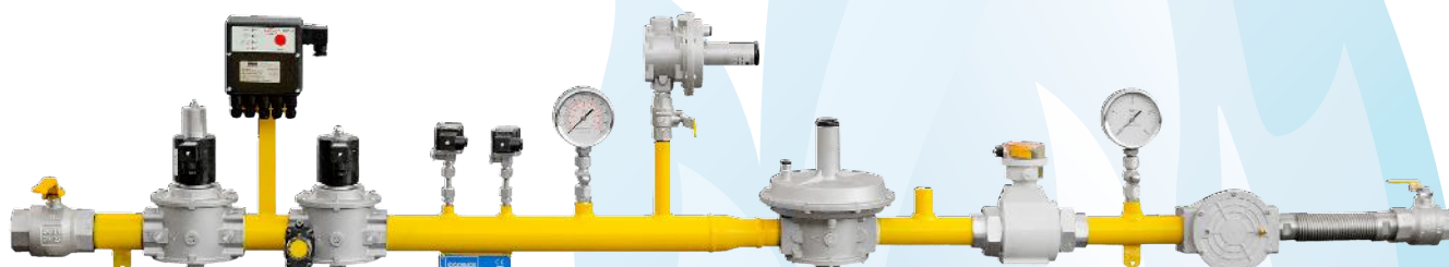
RAMPE GAS CON CONTROLLO DI TENUTA GAS TRAIN WITH TIGHTNESS CONTROL
